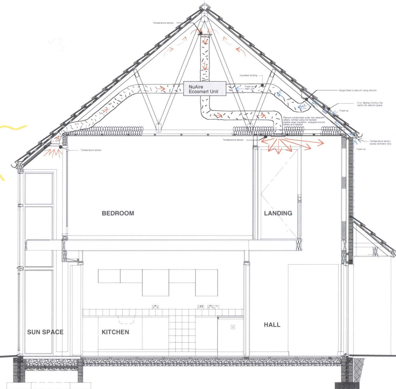
Cross Section 1:50
